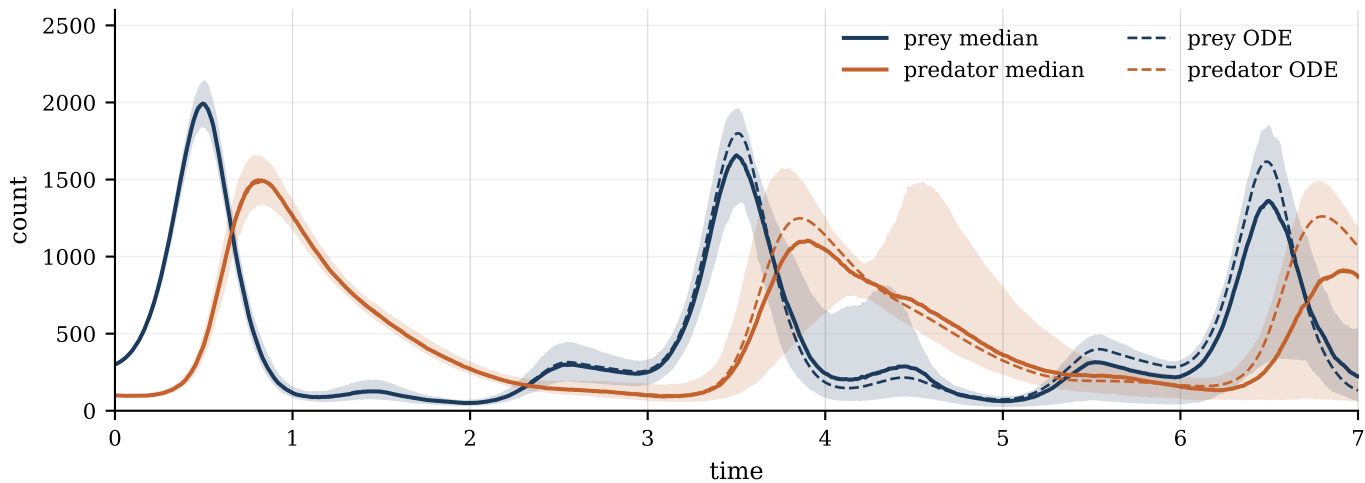
(c) median and 10-90% bands, 200 replicates, against the ODE
